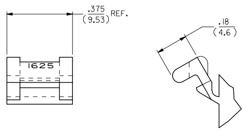
DETAIL B .062/(1.57) PREBENT MOUNTING EAR (SCALE 4:1)
